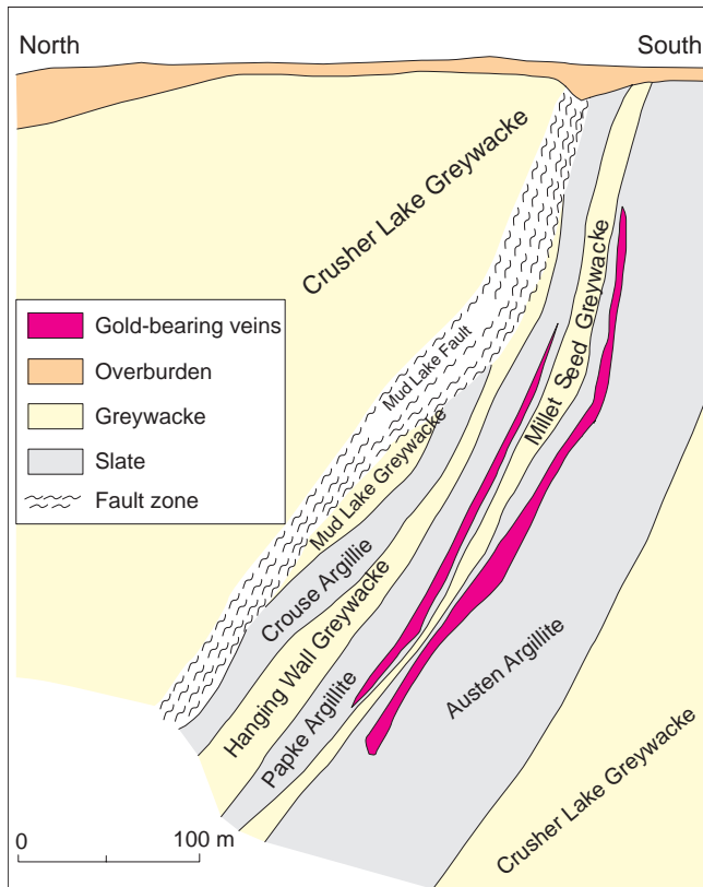
FIGURE 6. Section through an echelon gold veins at the Beaver Dam deposit, Nova Scotia (courtesy Seabright Resources Inc.).
