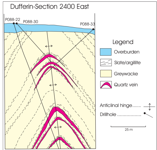
FIGURE 8. True stacked saddle reefs at the Dufferin extension deposit, Salmon River gold district. This deposit is the most recent discovery in the Meguma Group and is in production. It is the extension of the Old Dufferin Mine that has been faulted about 2 km north of the historic district, on a northwest fault (modified after Ryan and Smith, 1998).
