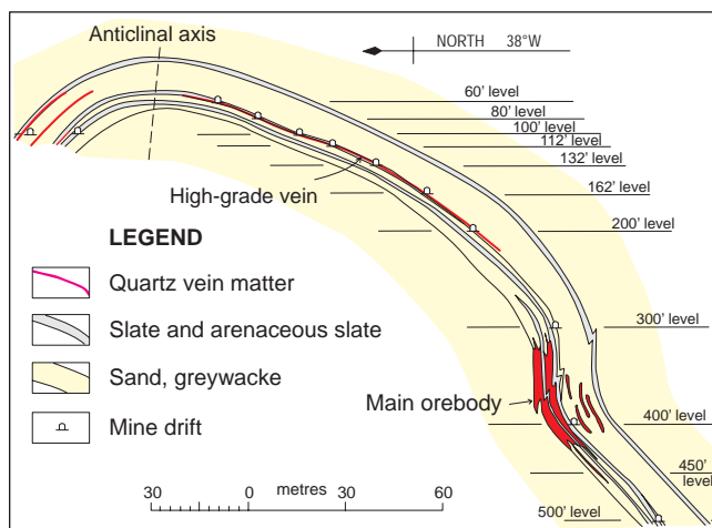
FIGURE 11. Geological section of the Caribou Mine, Nova Scotia. Note the two ore types: 1) a bedding-parallel, crack-seal vein in the upper part of the fold, and 2) quartz-healed breccia ore associated with a "kink" in the south flank of the fold (modified after Bell, 1948).
