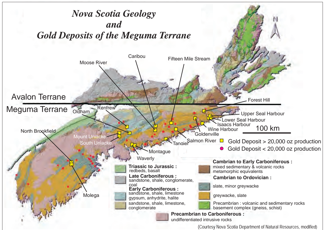
FIGURE 1. Regional geology of Nova Scotia and location of the 20 largest past-producing gold deposits. For smaller gold occurrences, the reader is referred to Malcolm and Faribault (1912) and Malcolm (1976) (courtesy Nova Scotia Department of Natural Resources).
