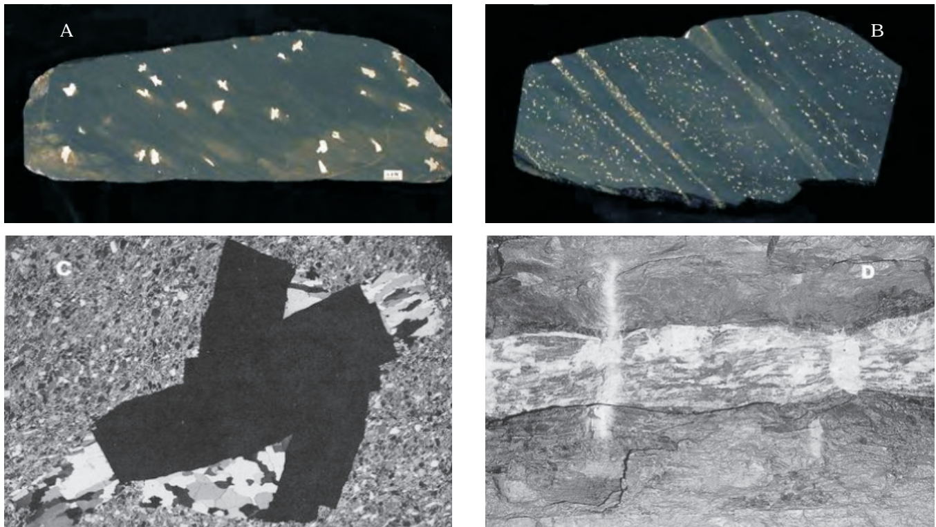
FIGURE 5. Geological features of Meguma gold Deposits. (A) Cruciform arsenopyrite crystals in metagreywacke from the Caribou deposit alteration aureole. Note lighter coloured silicification marbling the sample, particularly around arsenopyrites. (B) Bedding-parallel bands of disseminated arsenopyrite in black slate associated with veins at the Lawrencetown occurrence. Both lithologies in "A" and "B" may be auriferous. (C) Quartz pressure shadows on arsenopyrite crystals indicate crystallization prior to the last deformation. (D) Laminated "crack-seal" quartz (25 cm thick) from the Marker vein, Tangier mine. This is the most common vein-type and usually consists of laminated quartz overprinted by white bull quartz. (from Sangster, 1990).
