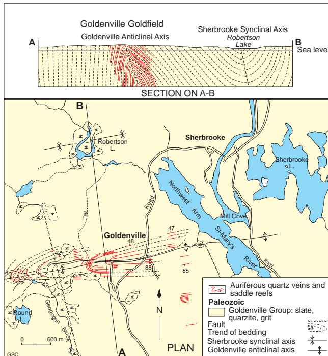
FIGURE 7. Geological plan of the Goldenville gold district. The best vein density occurred only on the western plunge of the culmination of the anticline (modified after Malcolm and Faribault, 1912).
