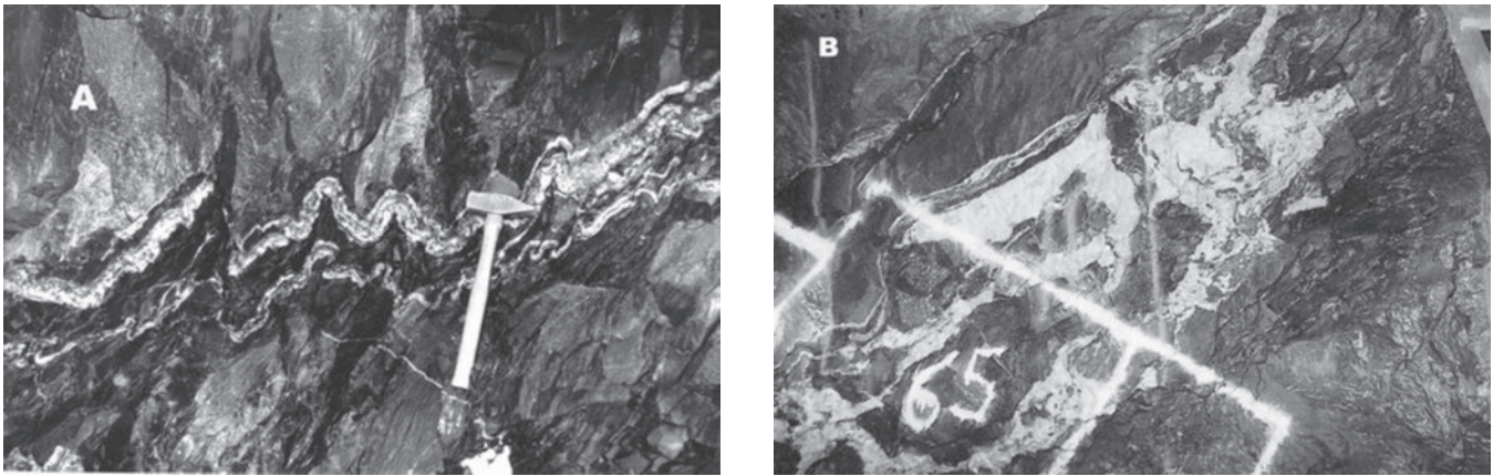
FIGURE 10. Geological features of Meguma gold deposits. (A) Twin vein, tangier gold district showing a pair of buckled, highly auriferous, quartz veins near the crest of the Tangier anticline. Also visible is the relationship of the veins to the overlying metagreywacke and underlying black slate. (B) Nugget vein, Tangier gold mine, showing chaotic quartz vein textures resulting from the development of superimposed, variably rotated en echelon veins in black, organic-rich, arsenopyrite-rich slate. Painted numbers are 25 cm high (from Sangster, 1990).
