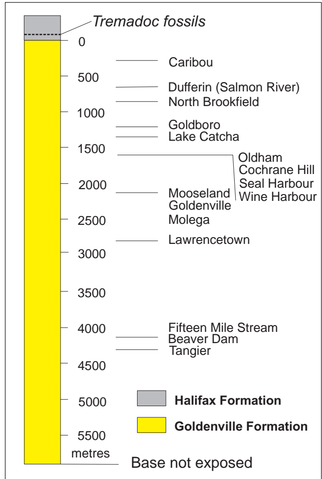
FIGURE 3. Stratigraphic location of selected gold deposits, Meguma Terrane, Nova Scotia. There is a concentration of occurrences at greater than 1500 metres and greater than 2000 metres below the upper Goldenville Formation contact, but these occurrences are widely separated and can not be demonstrated to be at the same stratigraphic horizon. Depths data was acquired by measuring the stratigraphic depth from sections on regional geological maps of Faribault (1898, 1901).
