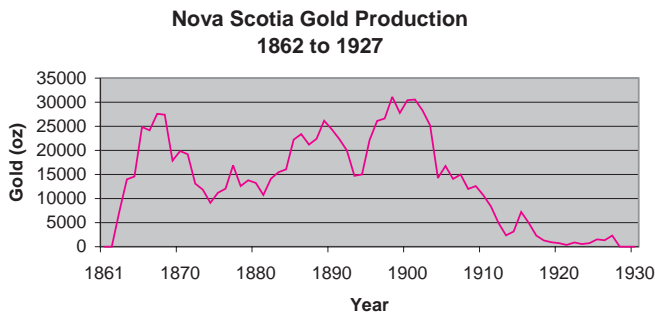
FIGURE 2. Nova Scotia Gold production, 1862 to 1927.
