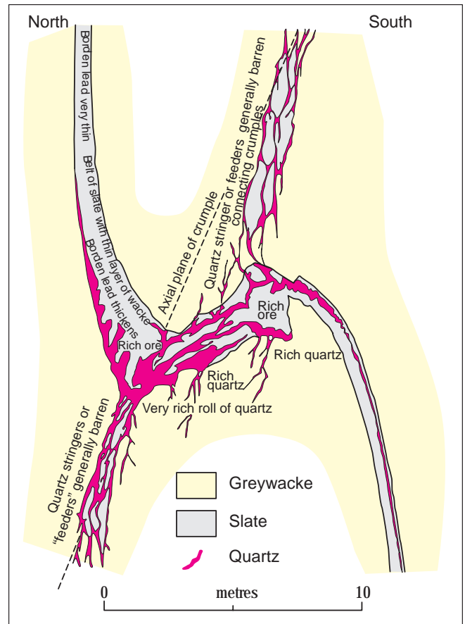
FIGURE 9. Geological section of a folded auriferous bedding-parallel vein intersected by a late barren vein breccia from the Mount Uniacke gold district. Note the gold enrichment in the bedding-parallel vein near the intersection with the late vein (after Malcolm and Faribault, 1912).
